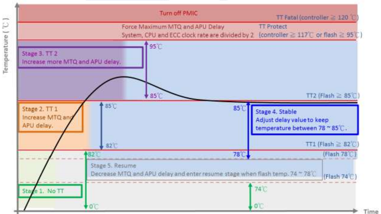
Figure 2-1 Thermal Throttling Schematic
